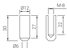
TERMINAL VARILLA ROSCADA M-8 Round screwing terminal / Borne rond à vis
